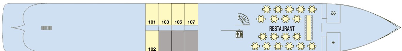
Main Deck
